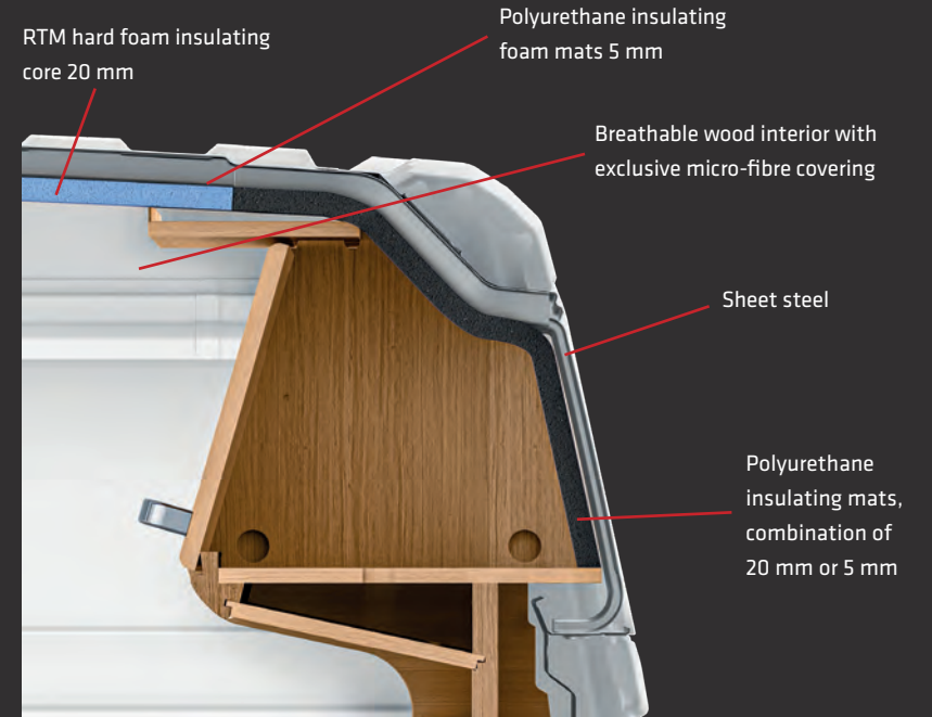
Malibu Van: elaborate main body insulation measures
