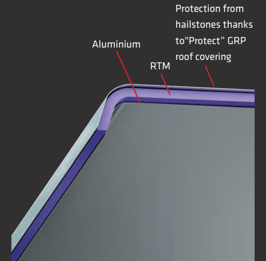
Malibu Van hybrid pop-up roof with the best insulation concept in its class in sandwich construction with light weight
